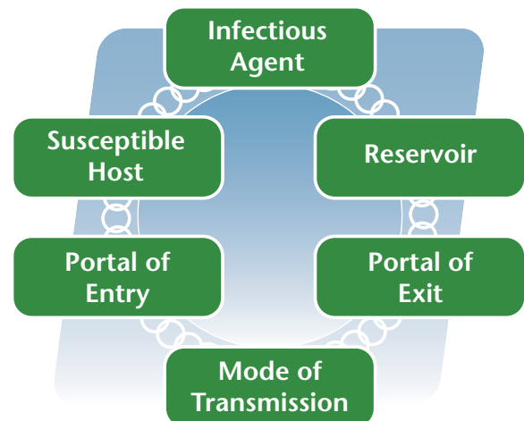
Figure 1: Chain of Infection – used with permission
