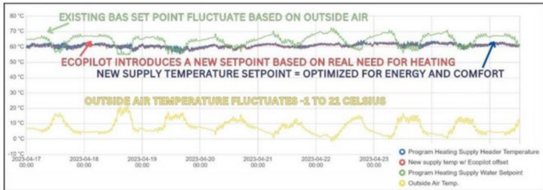
Figure 1 Every 2-minutes, iBOS® calculates the building balance point temperature and provides a new offset to the BAS based on ever-changing building variables. The result is energy savings while maintaining occupant comfort.
