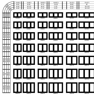
Casement Clad Combination Units - Elevation Chart
