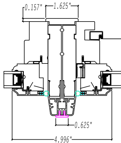
TRANSOM / CASEMENT CLAD MULL
