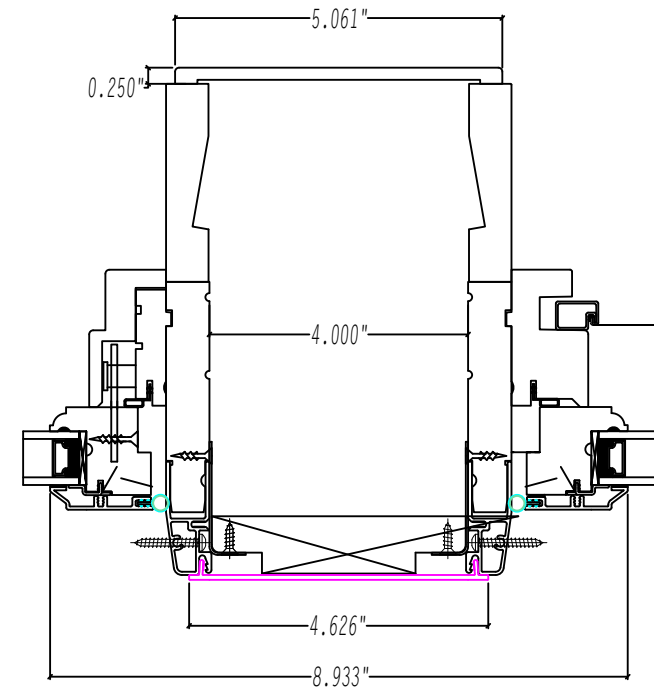
TRANSOM / CASEMENT CLAD MULL
