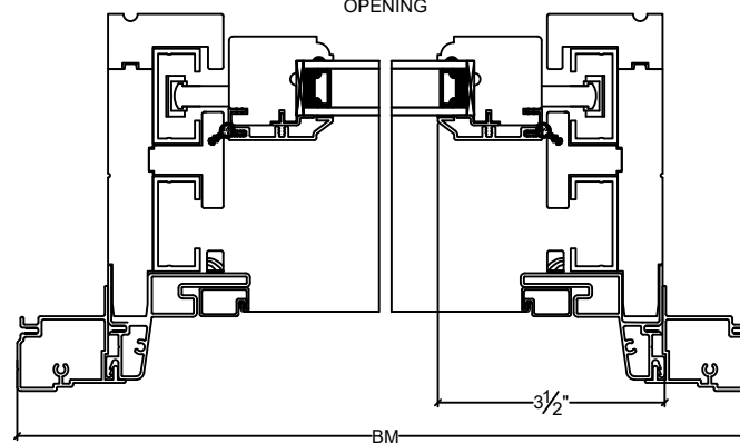
Bottom Sash
