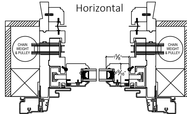
Top Sash
