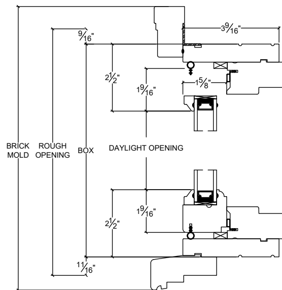
Vertical
