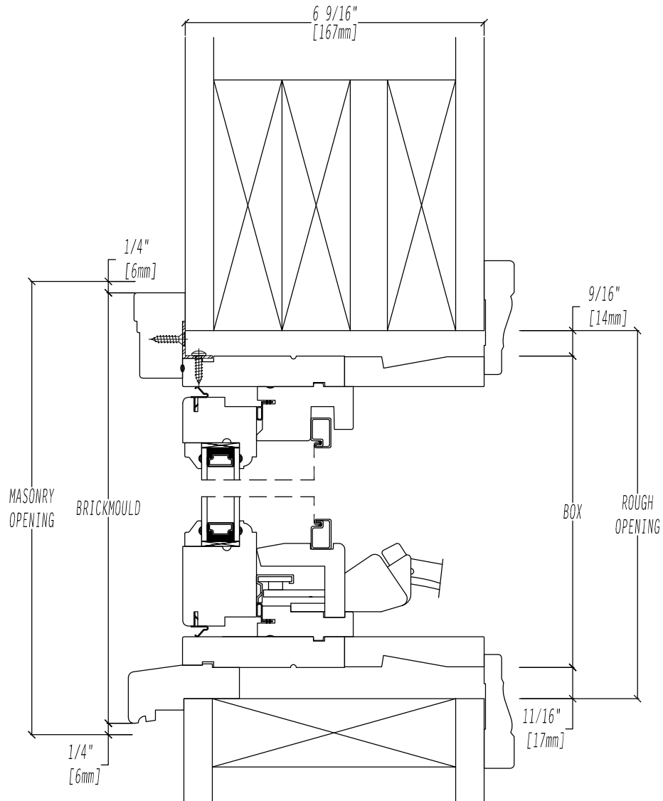
AWNING - TYPICAL WALL SECTION DETAIL
