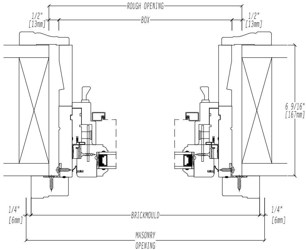
AWNING - TYPICAL WALL SECTION DETAIL
