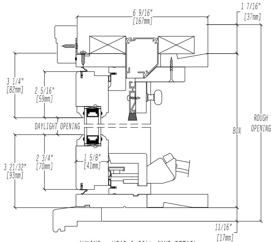
AWNING - HEAD & SILL JAMB DETAIL
