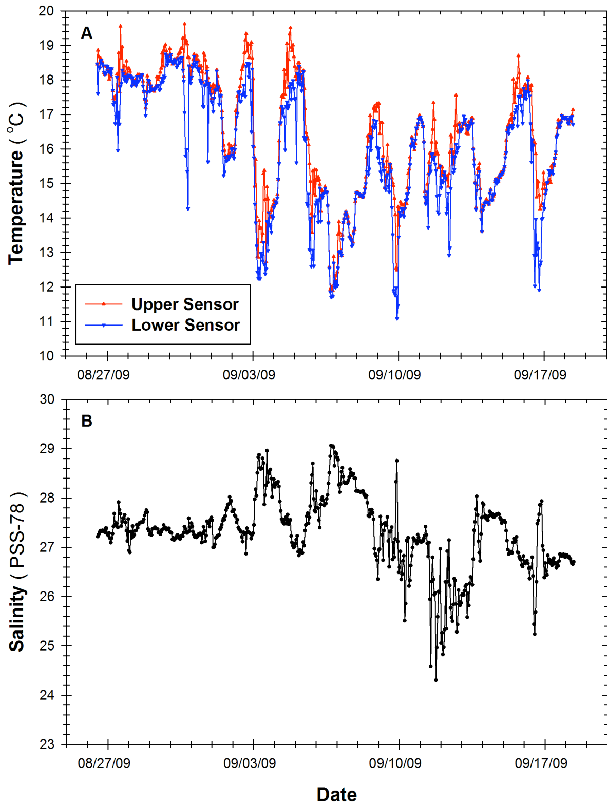
Figure 2. Environmental conditions at the mooring used for pCO 2 instrument deployments in Hood Canal, WA. Panel A: Water temperature from two RBR TR-1060 temperature loggers positioned above and below test instruments. Panel B: Salinity of water recorded by a SeaBird Electronics SBE 26 with 4M conductivity cell. All data sub-sampled at 1 h intervals corresponding to instrument sampling events.
